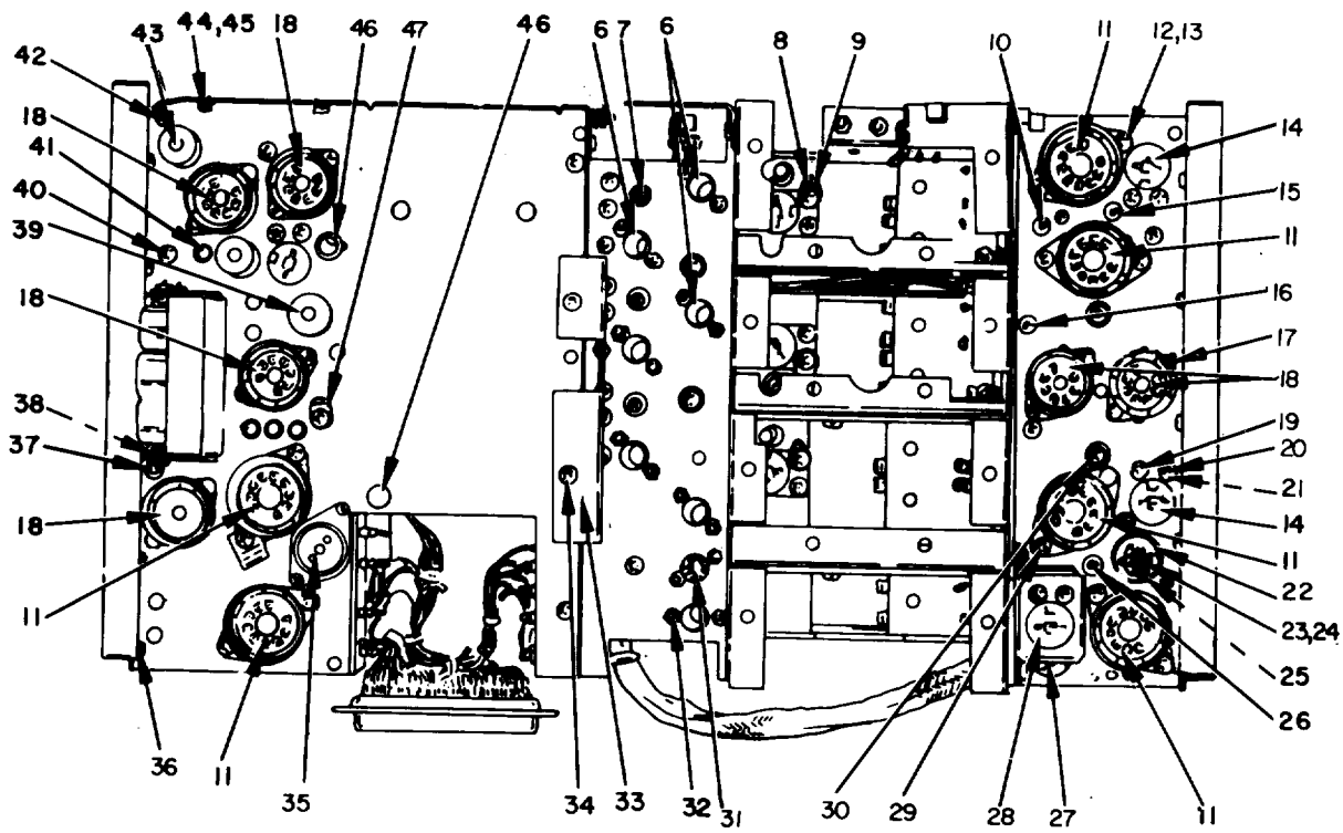
TOP VIEW 2
