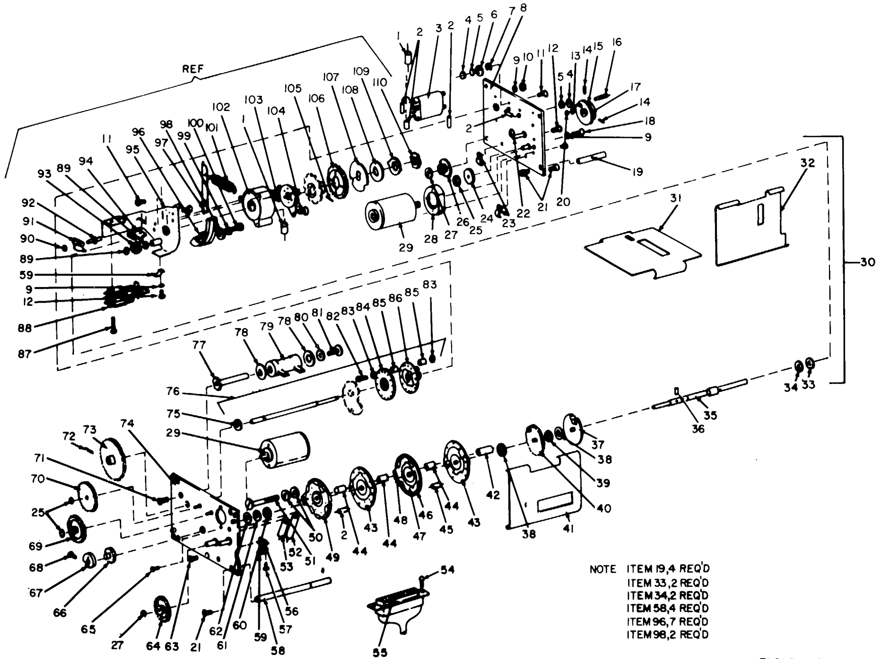
Figure 56. Autopositioner Submodule.
