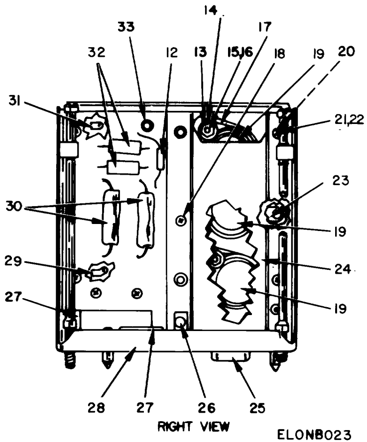
Figure 23. Amplifier.
