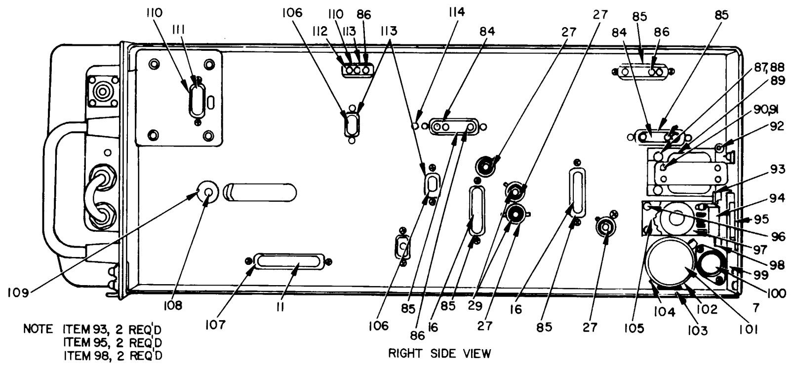
Figure 3. Chassis Assembly (Sheet 2 of 2).
