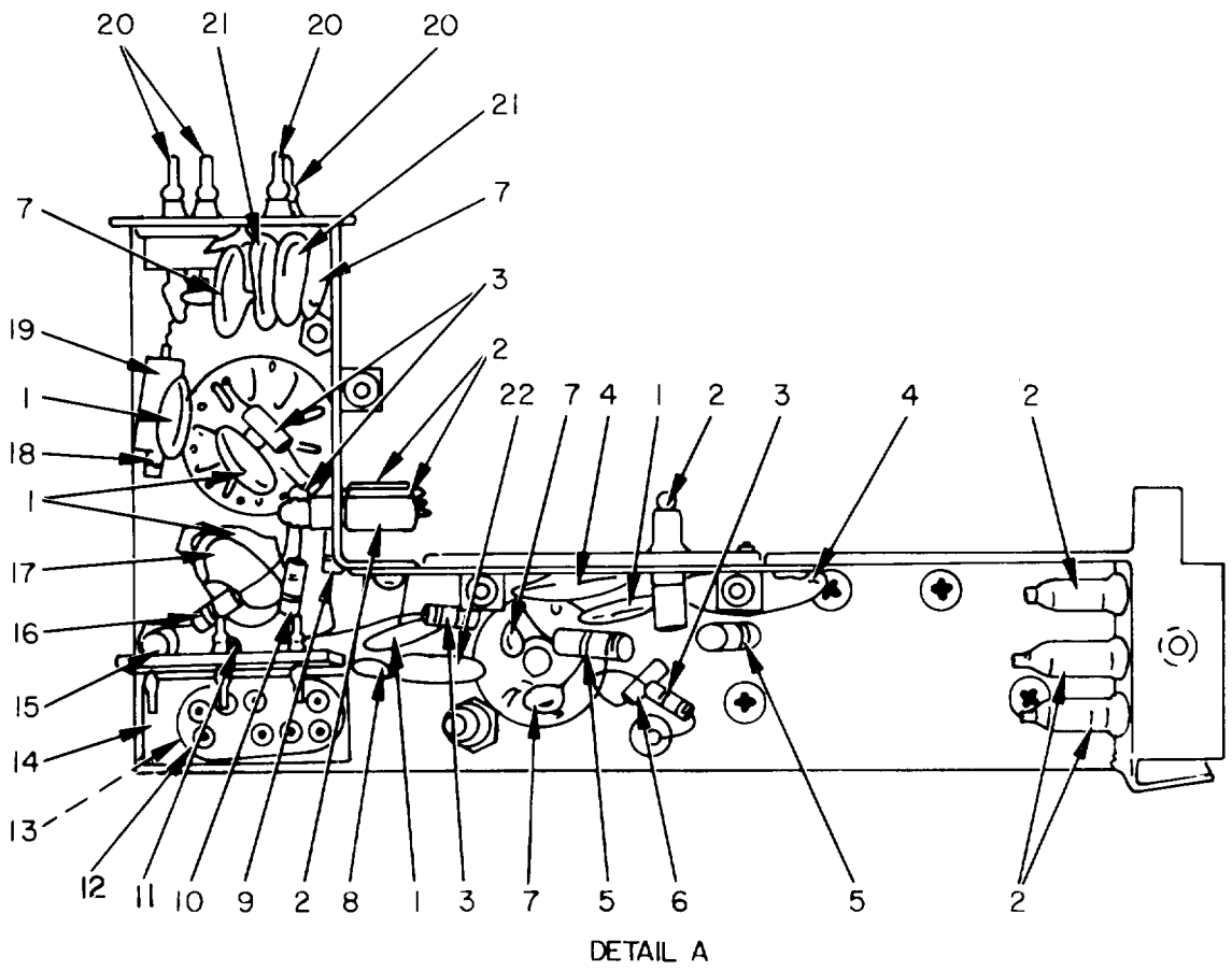
Figure 44. Radio Frequency Translator, Bottom View 3.
