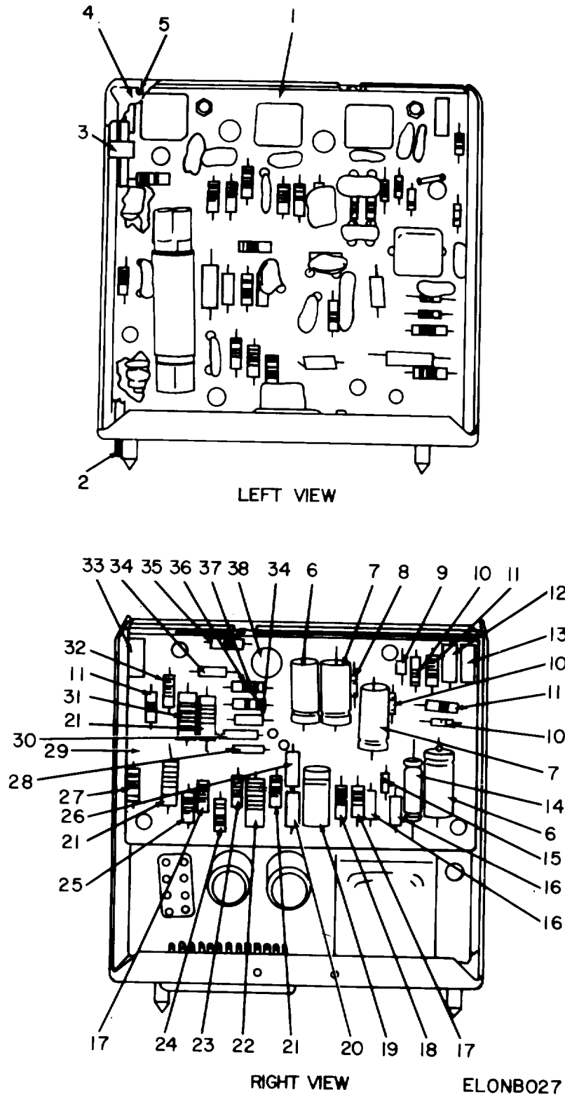
Figure 27. Audio Frequency Amplifier Module.
